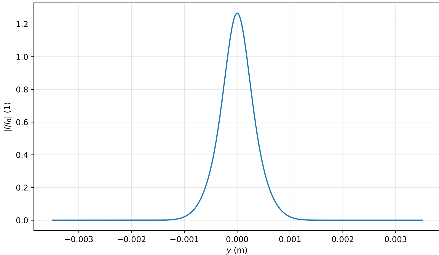
Intensity profile I(x=0, y, z=0.637)/I_0 , P_{in}=1.0P_{cr} , artificial time
